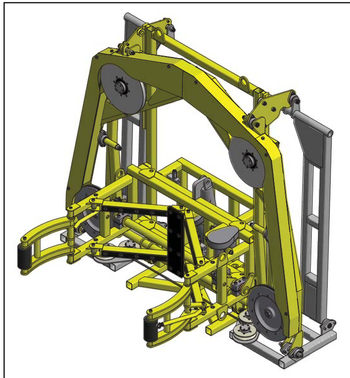
Diamond Wire Saw - Articulating
