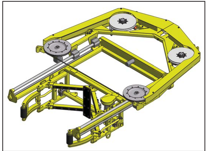
Diamond Wire Saw - In-line
